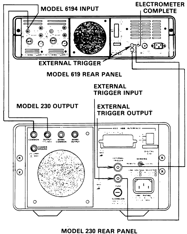
Figure 2-4. Using External Trigger
