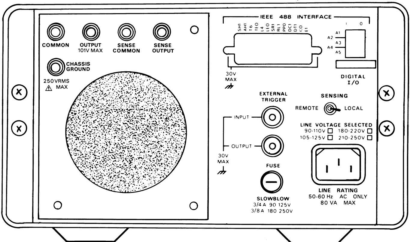
Figure 2-1. Model 230 Front and Rear Panel Controls and Connections
